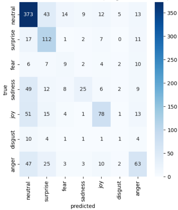
Confusion matrix with Focal Loss (weighted-F1=0.578)
